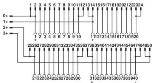
Connection scheme FLKM 50-PA-AB/OBN
